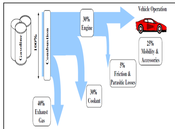
Fig 1: Energy Distribution for an IC Engine [3]
