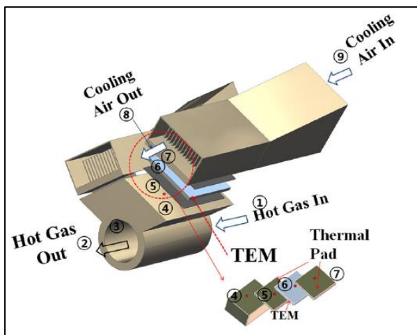
Fig 11: Conductive TEG Experimental System (TEGM 1) [8]
