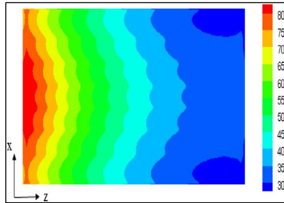
Fig 9: Cross sectional Temperature Distribution
